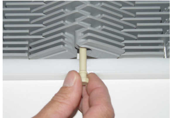
Insert rod For easy installation rod end must be beveled.
